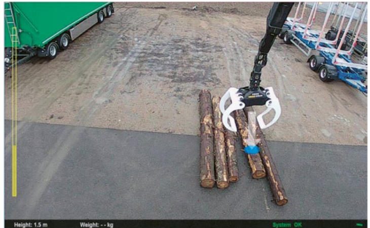
Screenshot from remote seat: The blue market dot indicating the crane head's location vertically, as well as the distance from the crane to logs are always visualised on screen.
